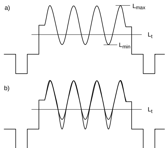
Fig. 2–14: Black-level-expansion
