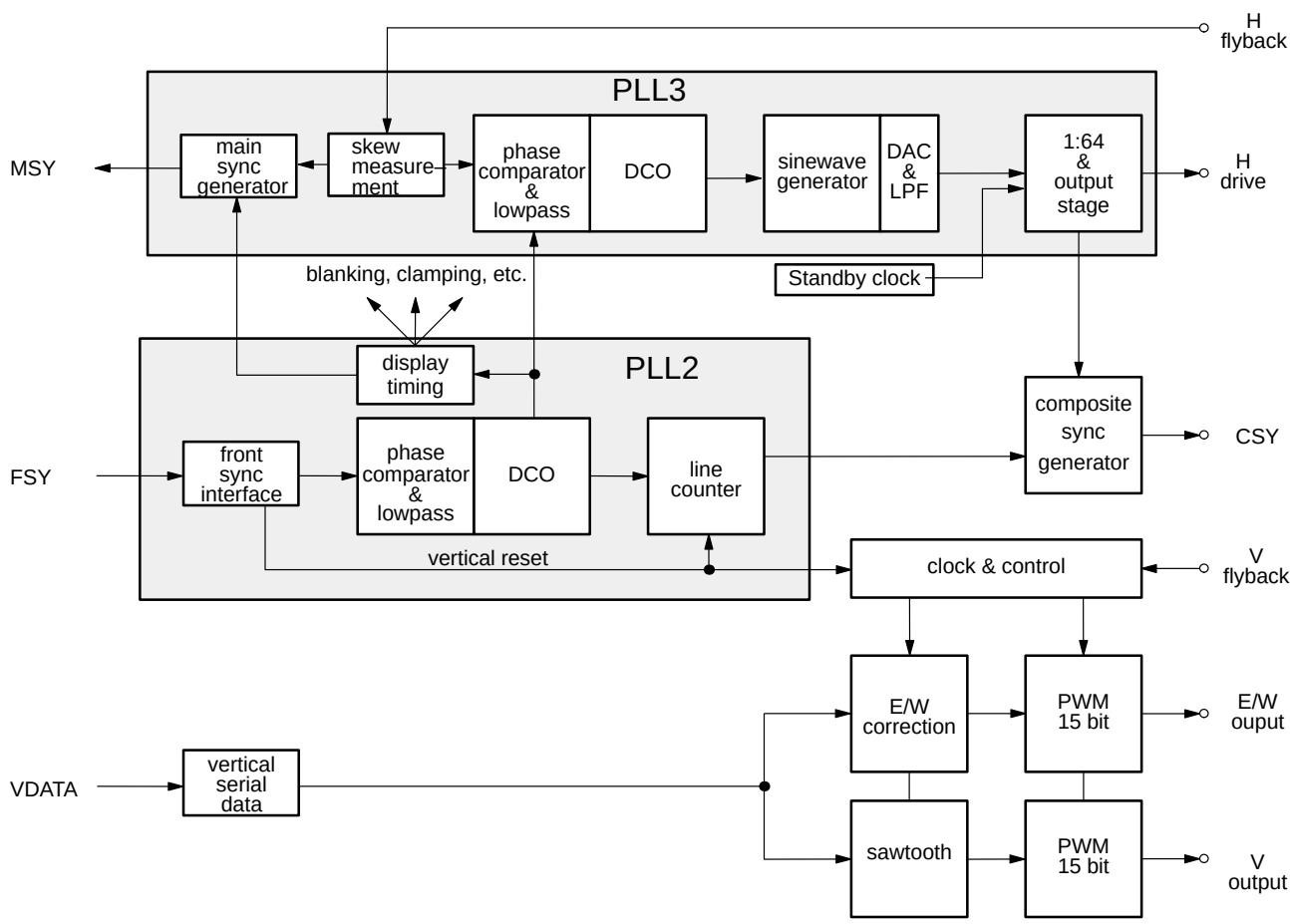
Fig. 2–28: Deflection processing block diagram
